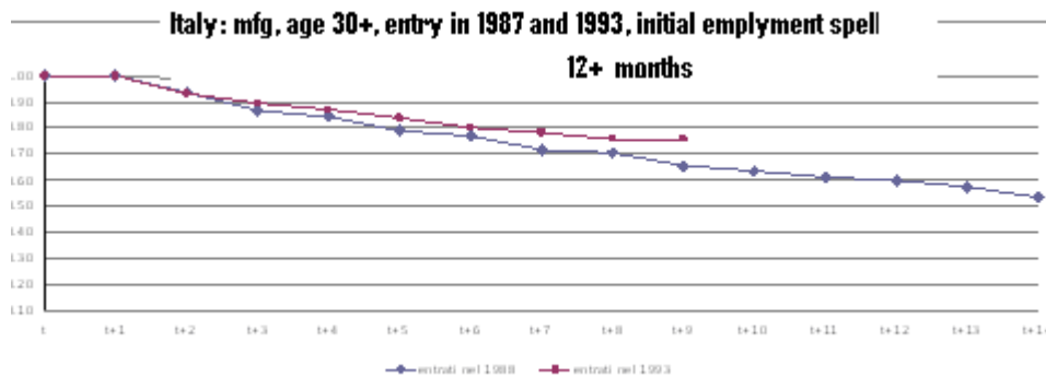
Fig. 4 – 6 - Survival curves: selected cohorts by industry, geography, year-of-entry, initial spell duration.
