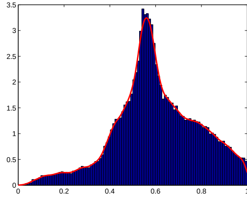
Figure 6: Posterior distribution of the learning parameter \beta with Gaussian density estimation of the likelihood and MCMC sampling. 400,000 simulations of 1,500 trading days each are performed. 1,500 pseudo-true trading days are assumed to be observed. The pseudo-true value is \beta = 0.55 .
