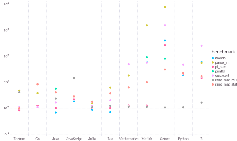
Figure 2: Smaller is better: the benchmark times for operations implemented in a number of programming languages relative to C, whose performance time is set to 1.0. From http://julialang.org/benchmarks/ .
