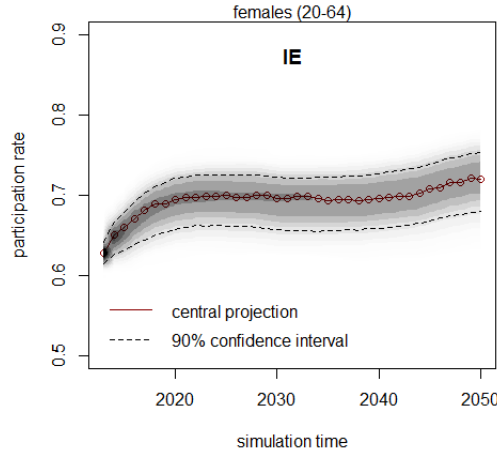
Figure 6: Quantifying forecast error due to parameter uncertainty, using JAS-mine’s regression utility tools to bootstrap regression coefficients during a multi-run execution of a simulation over 1000 runs. The chart was produced using kernel density estimation from analysis of the simulation’s output database performed by the statistical software program ‘R’.
