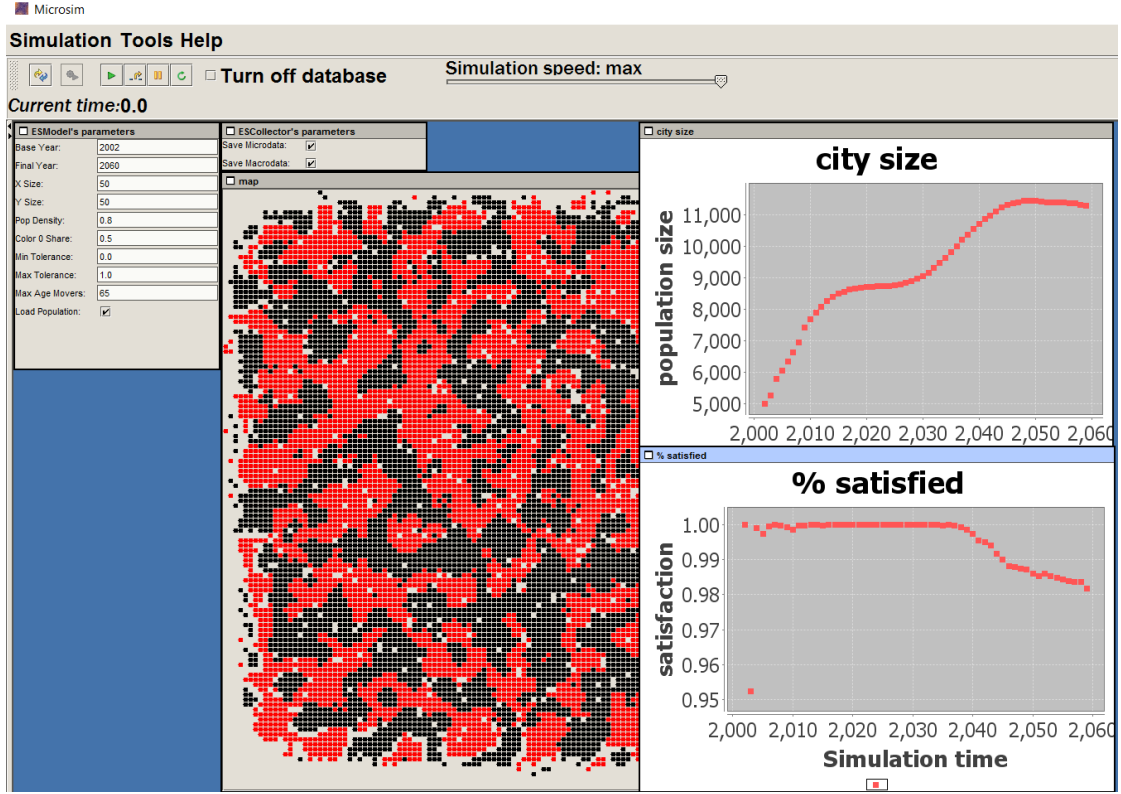
Figure 7: Interactive Mode: screenshot of the JAS-mine graphical user interface showing output from the Extended Schelling demonstration model, available at www.jas-mine.net/demo/extended-schelling .
