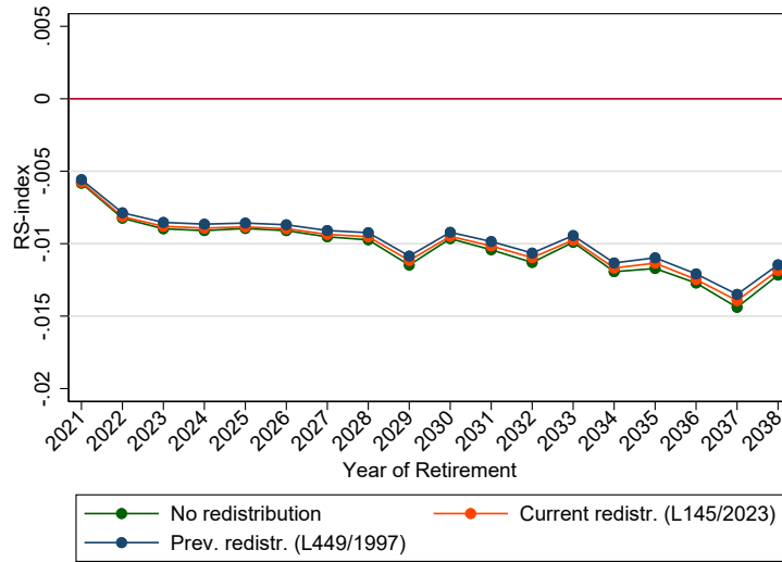
Figure 6: RS-index with alternative indexation
