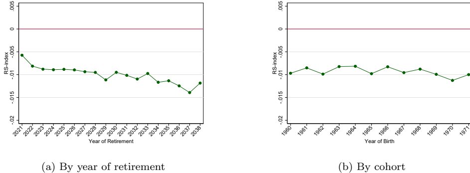
Figure 4: RS-index
